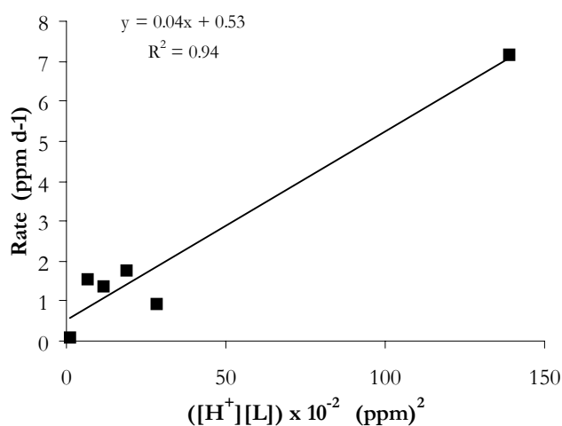
Figure 3b: Correlation of rate of formation of lycopene with the product of concentrations of hydrogen ion and lycopene at the ambient temperature ripening. The R^2 value and the linear least square fit equations are given in the figures
