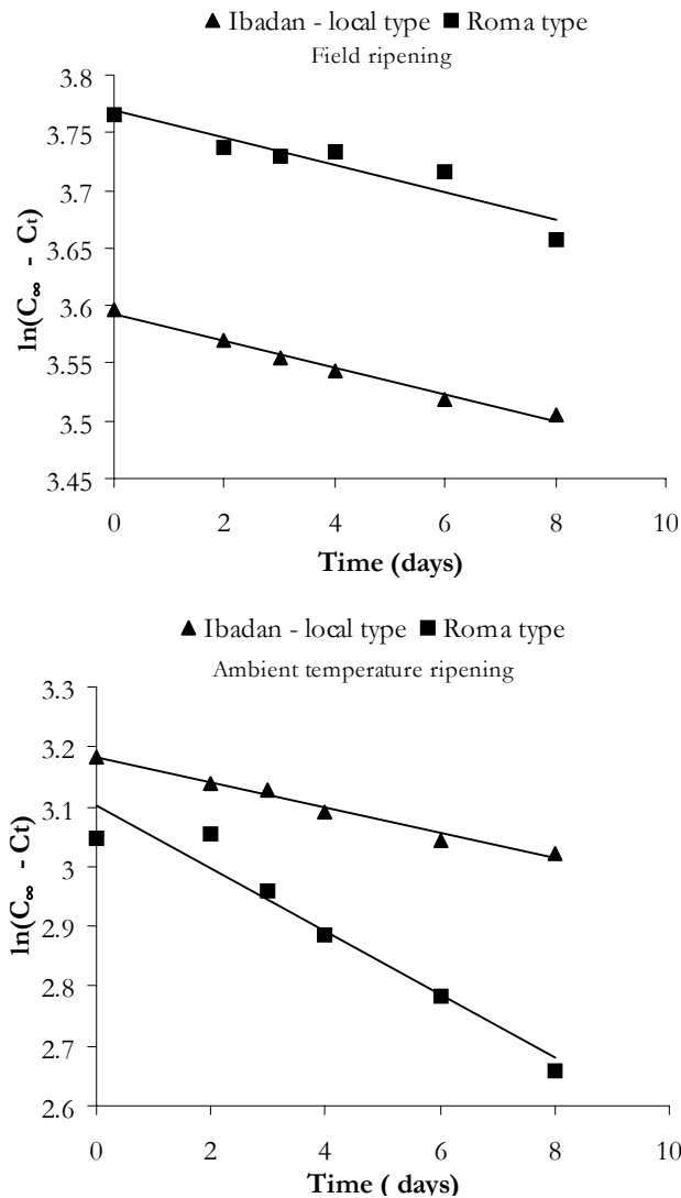
Figure 1: Plot of \ln(C_\infty - C_t) against time under the field and ambient temperature ripening
